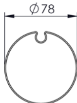
Rullo - Tube
